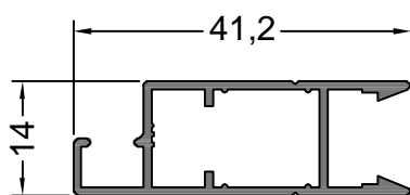
12005 0.322 Kg/m CORREDIZA MOSQUITERO HOJA
